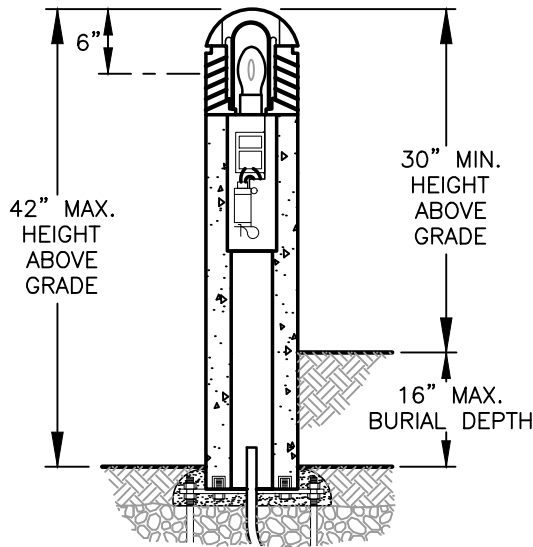
SINGLE FUNCTION LUMINAIRE
