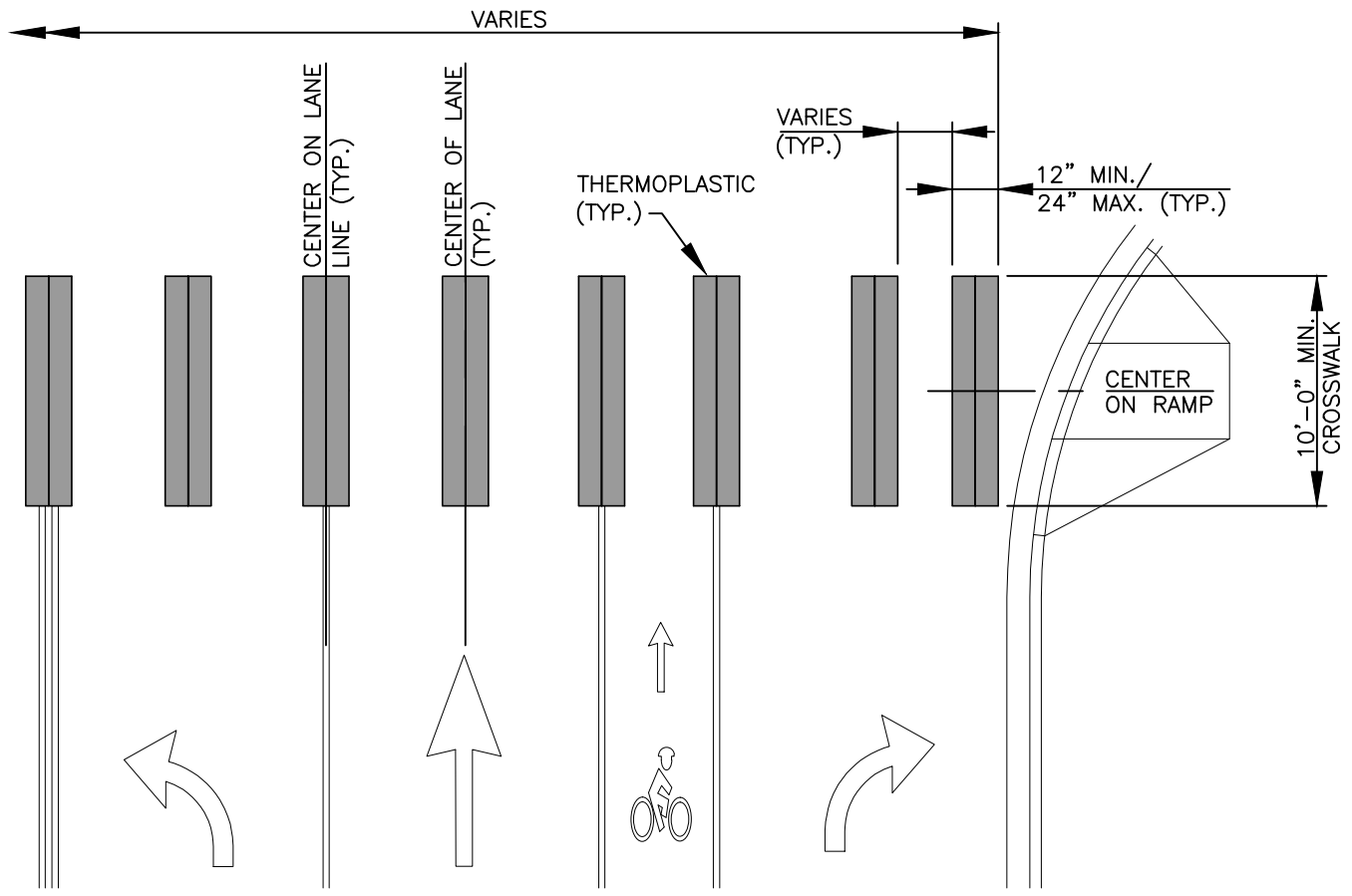
STANDARD CROSSWALK
