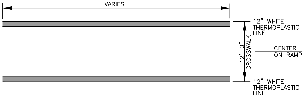
CROSSWALK ALTERNATE
