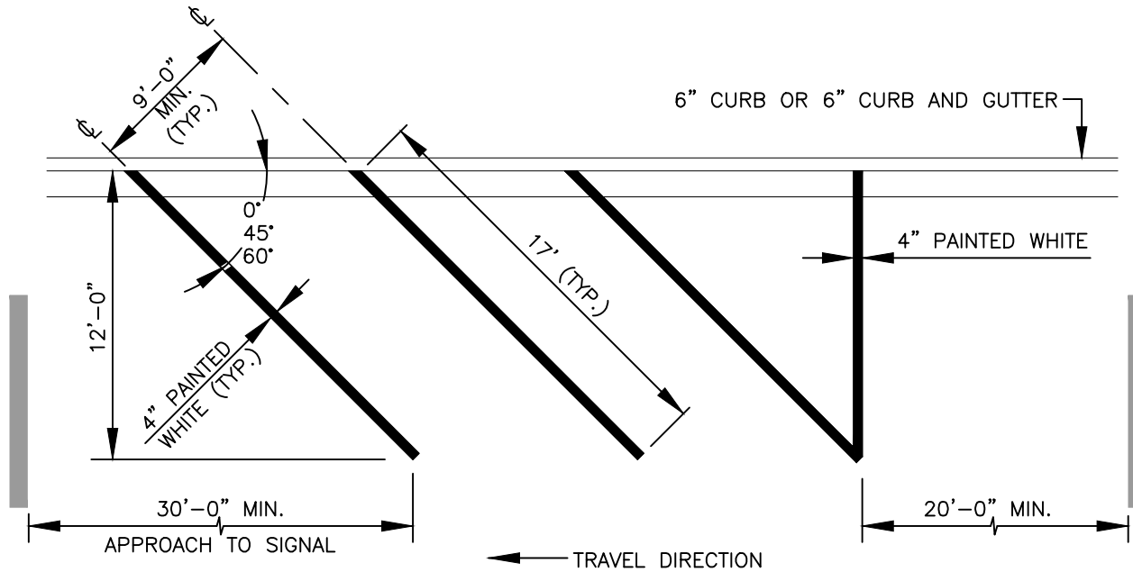
ANGLE PARKING STRIPE
