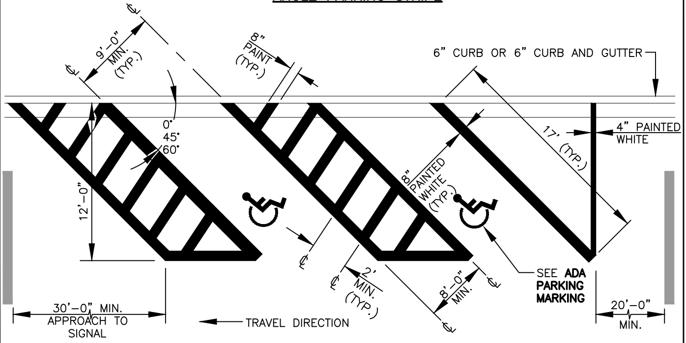
ADA ANGLE PARKING STRIPE
