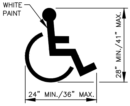
ADA PARKING MARKING
