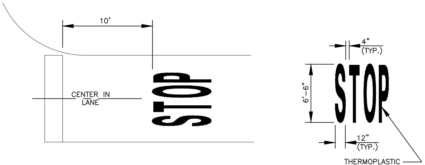
"STOP" PAVEMENT LEGEND
