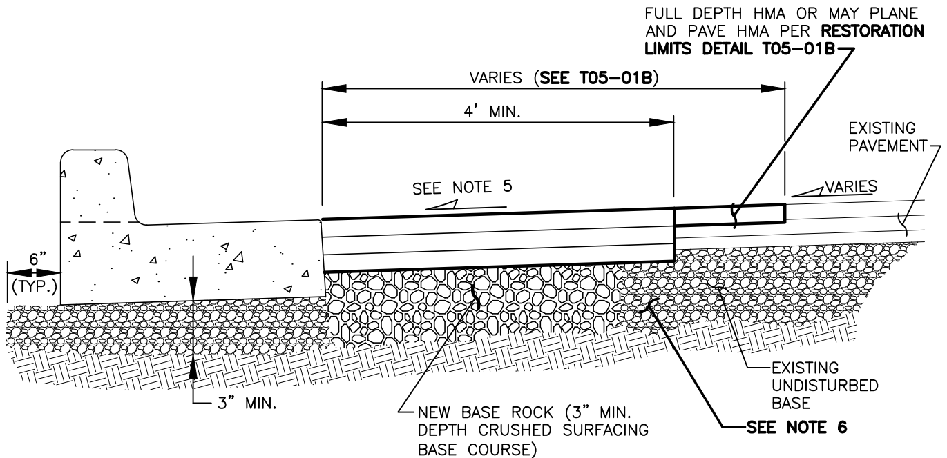
TYPE E-1 CURB
