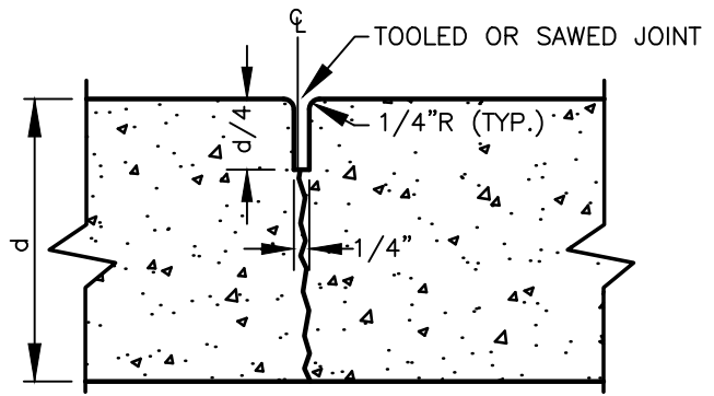
CONTRACTION JOINT
