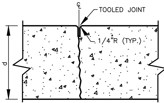
SURFACE JOINT
