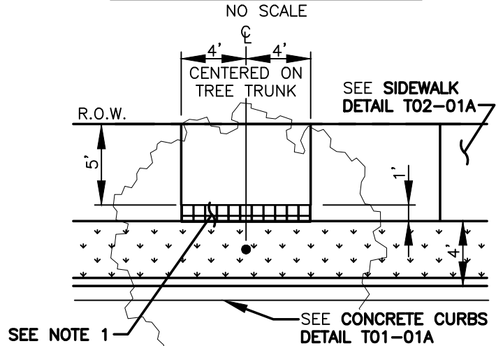
GREEN NECKLACE NORTH AND COMMERCIAL STREET: PAVER AT TREE WELL
