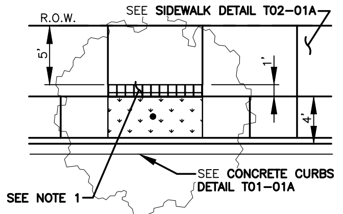
GREEN NECKLACE NORTH AND COMMERCIAL STREET: PAVER AT TREE WELL
