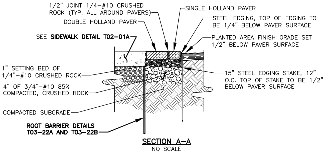
GREEN NECKLACE NORTH: PAVER AT PLANTER STRIP NO SCALE
