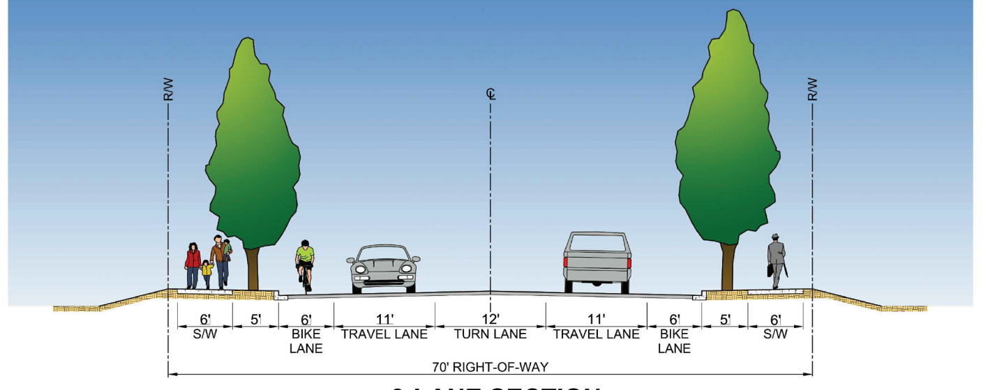
3-LANE SECTION
