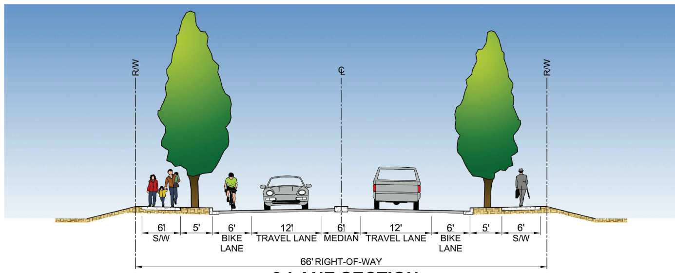
2-LANE SECTION
