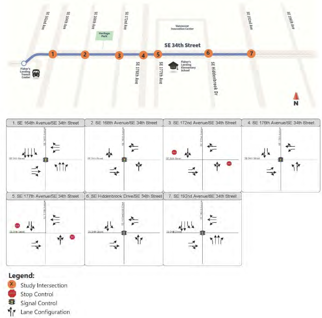
Figure 3. With Repurposed Lane Configurations
