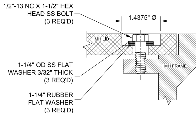
BOLT DOWN DETAIL
