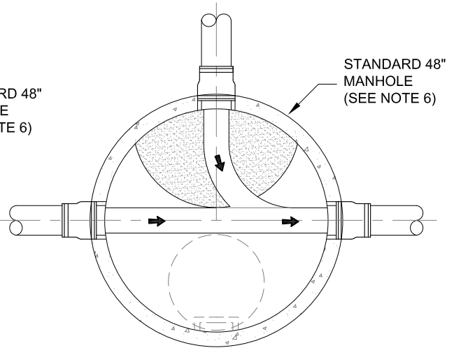
BRANCH FLOW PLAN VIEW
