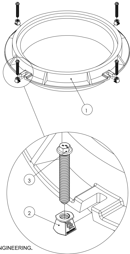
DETAIL A
