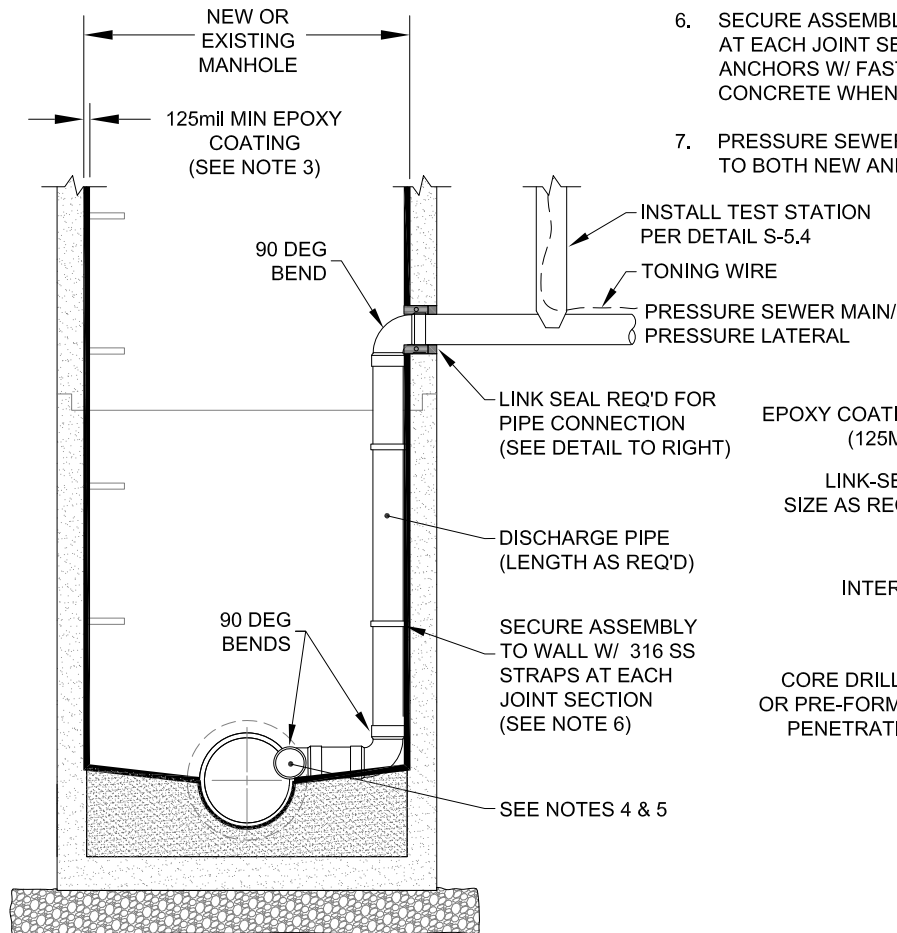
PROFILE VIEW
