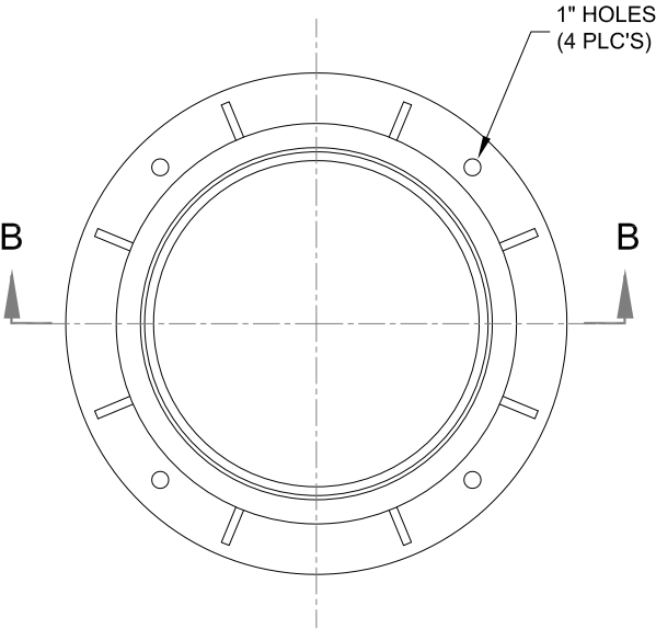
COMPOSITE MANHOLE FRAME PLAN VIEW
