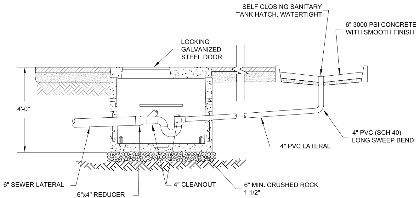
PROFILE VIEW
