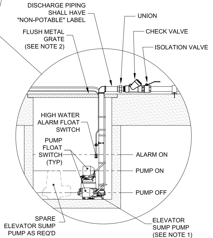
DETAIL VIEW
