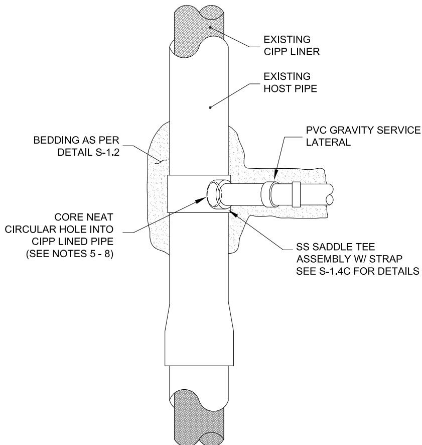
PLAN VIEW
