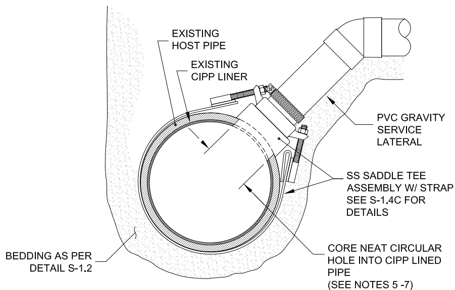
PROFILE VIEW
