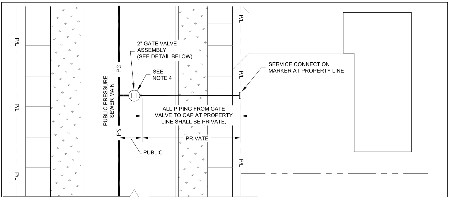
PLAN VIEW
