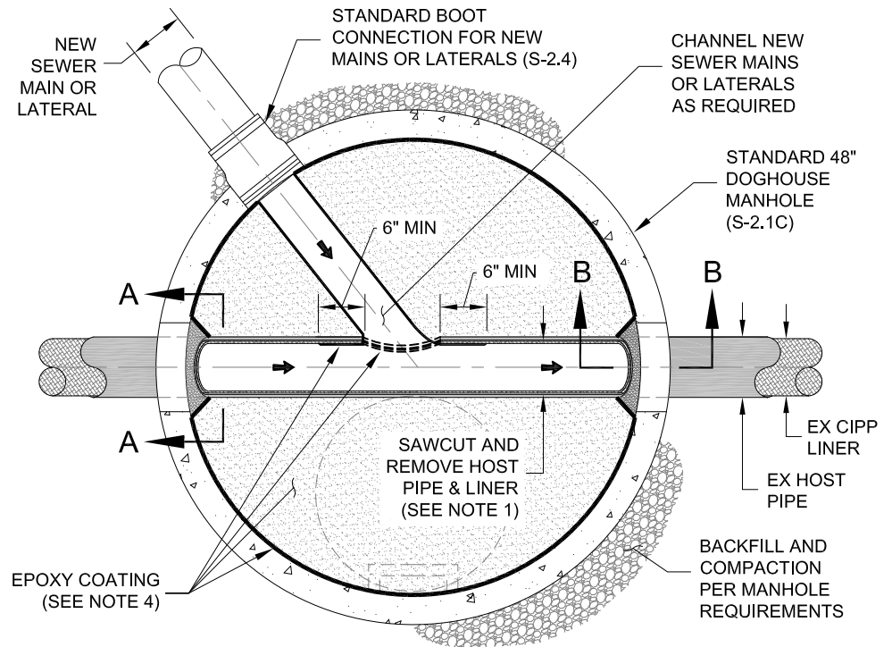
MANHOLE CONNECTION PLAN VIEW
