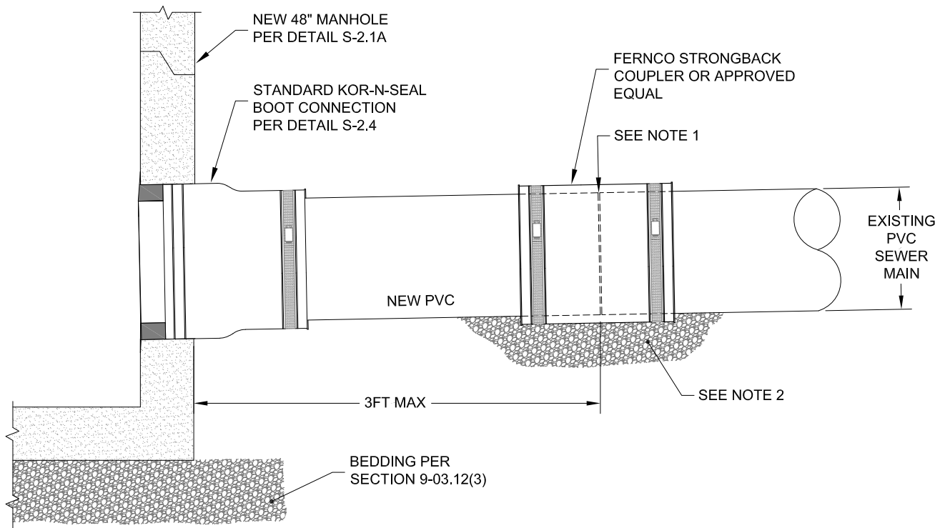
PROFILE VIEW
