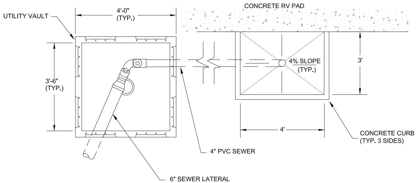
PLAN VIEW
