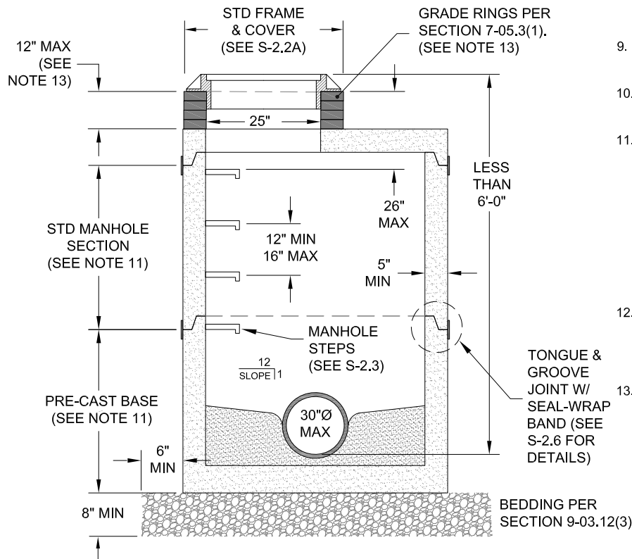
PROFILE VIEW
