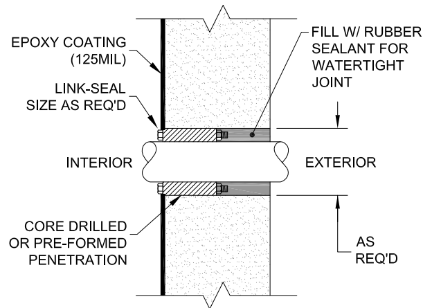
LINK-SEAL DETAIL
