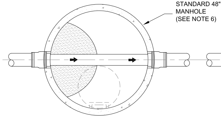
THROUGH FLOW PLAN VIEW
