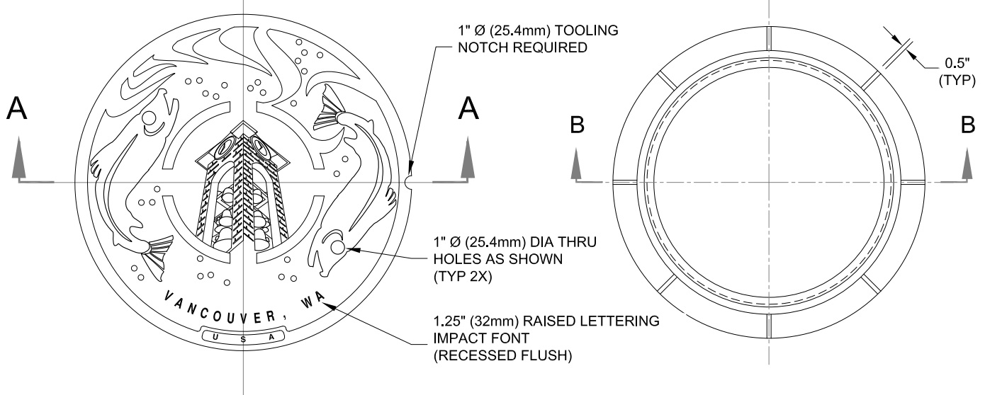
SUBURBAN MANHOLE FRAME PLAN VIEW
