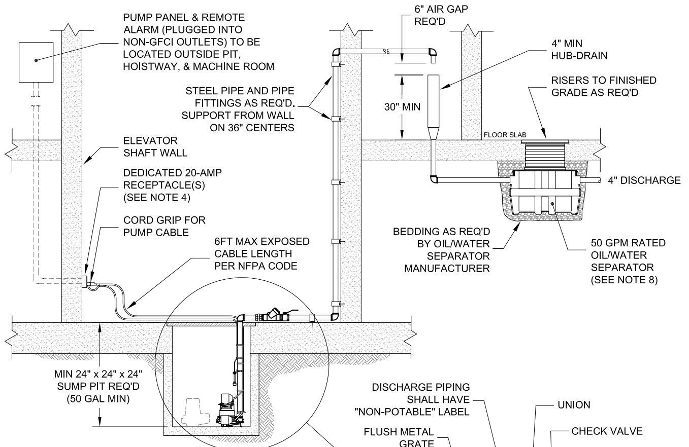
PROFILE VIEW
