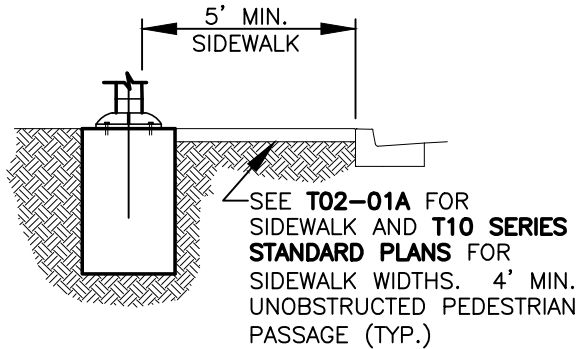
ATTACHED SIDEWALK OPTION 1
