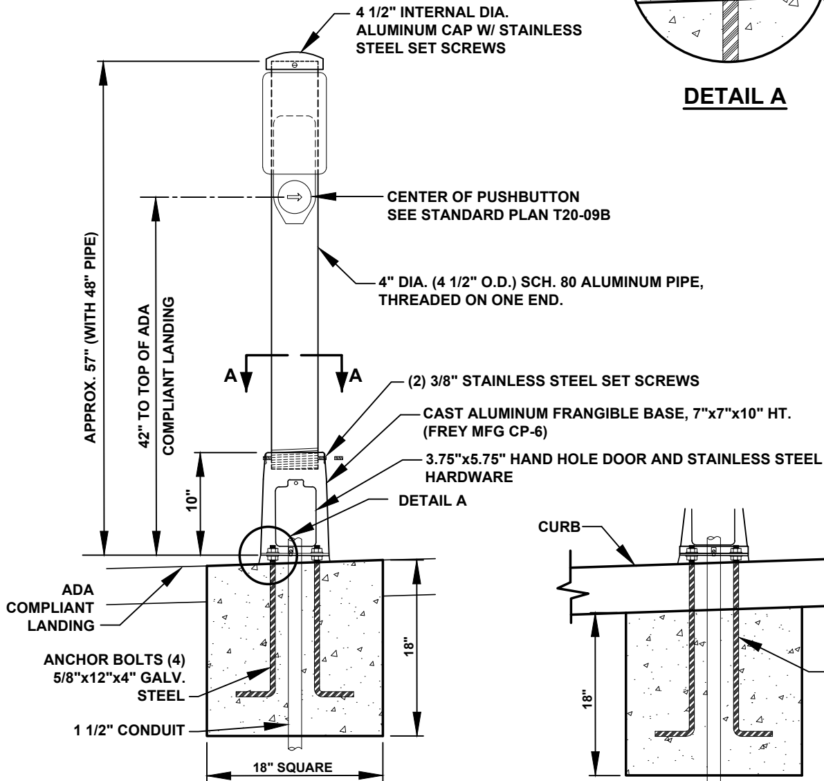
FOUNDATION
